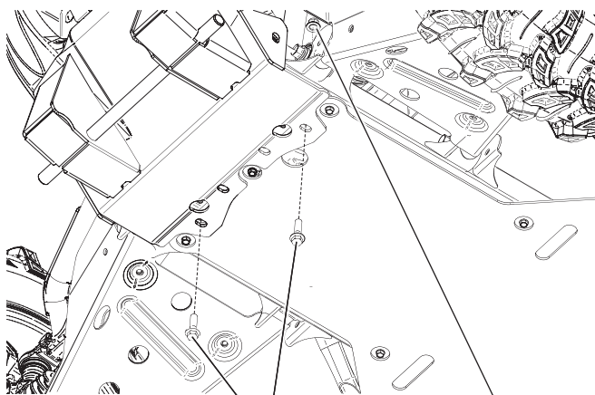
M10 - 1.25 × 35 mm HEX FLANGE BOLT
